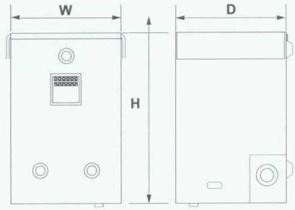
Style 2 - Non-Encapsulated
