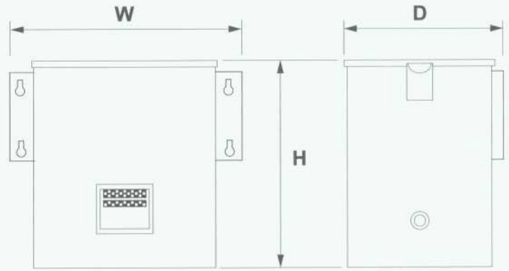
Style 4 - Encapsulated
